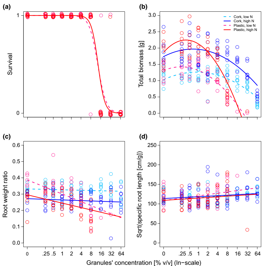
FIGURE 2 Relationships of (a) survival; (b) total biomass; (c) root weight ratio; and (d) specific root length of plants of Plantago lanceolata grown at different concentrations of the plastic ethylene propylene diene monomer (EPDM) and cork granules, and under low and high nutrient (N) conditions. Each circle represents a single data point (plant), and the fitted lines are from (generalized) linear models. Because in the presence of cork granules all plants survived, only survival in the presence of plastic granules is shown
